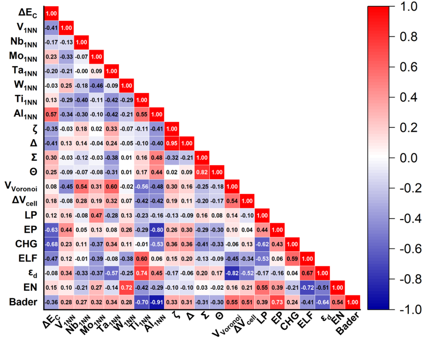
Fig. 4 The Pearson correlation coefficient (PCC) between all descriptors except the 2NN and 3NN composition around the dopant C and the carbon doping energy ( \Delta E_C ).
