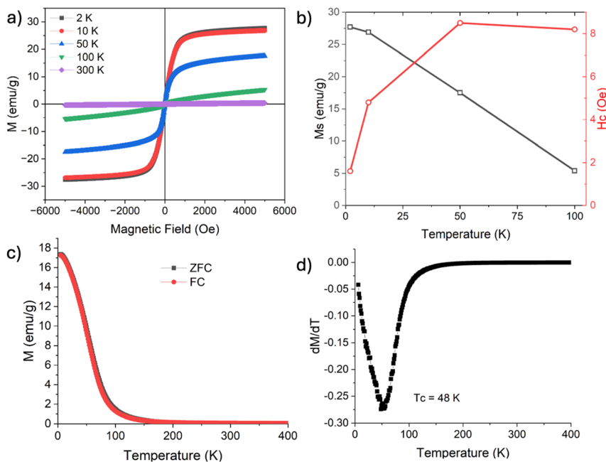
Fig. 6 Magnetic behaviour of the solution-annealed (SA) condition. (a) Isothermal magnetization ( M - H ) loops measured at multiple temperatures, showing ferromagnetic behaviour at low temperature and a paramagnetic behaviour at room temperature. (b) Temperature dependence of saturation magnetization ( M_s , left axis, black squares) and coercivity ( H_c , right axis, red circles). (c) Zero-field-cooled (ZFC) and field-cooled (FC) magnetization curves measured in a 1000 Oe applied field, revealing a single magnetic transition. (d) Derivative of magnetization ( dM/dT ) used to determine the Curie temperature, T_c \approx 48 K.
