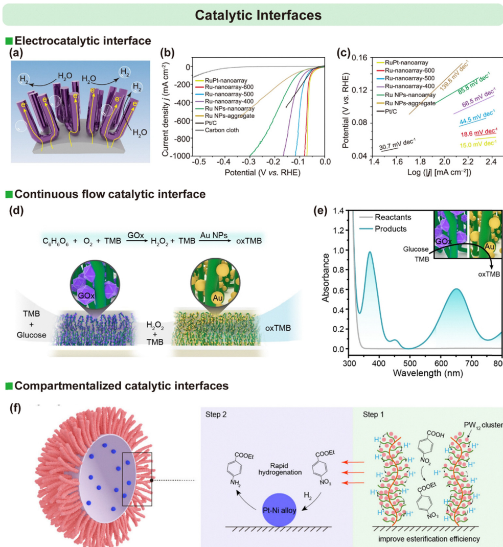
Fig. 17 (a) Schematic representation of a metallic Ru nanoarray designed for the hydrogen evolution reaction (HER). (b) iR -corrected polarization curves in 0.5 M H 2 SO 4 solution for alloy RuPt nanoarray, metallic Ru nanoarray- T , Ru NP nanoarray, Ru NP aggregates, commercial Pt/C-decorated carbon cloth, and pristine carbon cloth. (c) Tafel plots derived from the polarization curves shown in (b). Reproduced from ref. 54 with permission from Springer Nature, Copyright 2025. (d) and (e) Illustration and UV-vis spectra for a cascade reaction in PBS (pH 5.05) sequentially catalyzed by GOx-functionalized micellar brushes and Au NP-functionalized micellar brushes. Reproduced from ref. 51 with permission from Wiley, copyright 2021. (f) Schematic diagram of the sequential tandem conversion of p -nitrobenzoic acid within a microreactor engineered via surface modification strategies. Reproduced from ref. 55 with permission from Wiley, copyright 2025.
