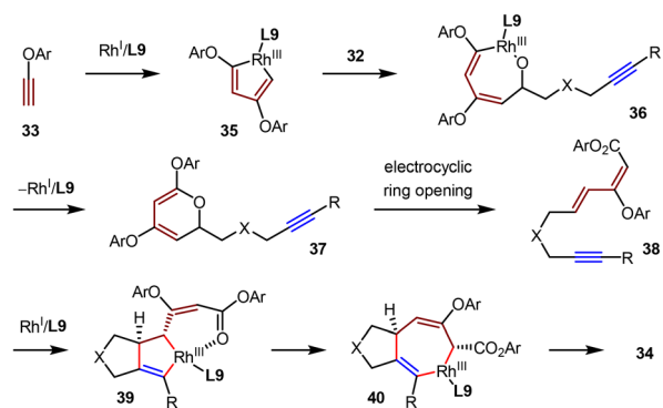
Scheme 12 \text{Rh}(\text{I})/(\text{R})\text{-H}_8\text{-BINAP} -catalyzed intermolecular [2+2+2] trimerization/asymmetric intramolecular [4+2] cycloaddition.
