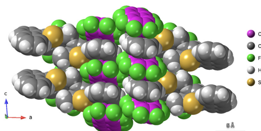
Fig. 7 Co-crystal of 1,2-bis(2-methyl-5-(1-naphthyl)-3-thienyl)perfluorocyclopentene 9o with perfluoronaphthalene 10 , CSD code CIXBAN02. 65
