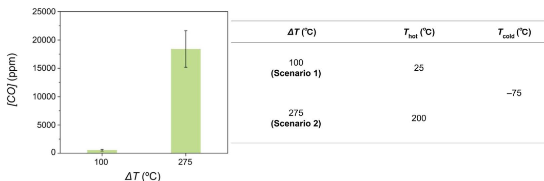
Fig. 6 Simulation of thermoelectrically powered reactive carbon electrolyzer on Mars. The plot shows the variation of [CO] at two ΔT values. The T hot was controlled by placing one face of the TEG in contact with a hotplate, and the T cold was controlled with a dry ice-ethanol bath placed in contact with the opposite face of the TEG. The [CO] was recorded after ΔT reached a steady state and thermoelectric-driven electrolysis was ran for 10 minutes. The table presents two possible scenarios to achieve those two ΔT values. Scenario 1 represents human settlement on Mars and Scenario 2 represents travel to Mars. The error bars represent the standard error from n = 3 independent experiments.
