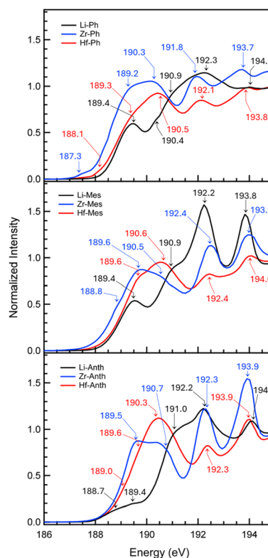
Fig. 7 B K-edge XAS spectra of [\text{M}(\text{RBH}_3)_4] complexes with \text{M} = \text{Zr} (blue) and Hf (red) and comparison to their corresponding Li( \text{RBH}_3 ) salts (black). Labeled positions indicate peak maxima in the spectra or peak positions identified by analysis of the second derivative traces (Fig. S51–S53; SI).
