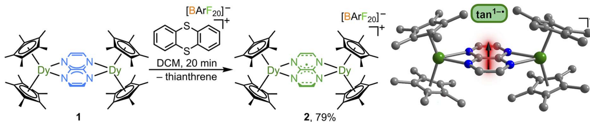
Fig. 4 Synthesis of [(Cp^*_2Dy)_2(\mu-tan')][BARF_{20}] (2) through oxidation of [(Cp^*_2Dy)_2(\mu-tan)] (1) with [Thian^{\cdot+}][BARF_{20}] (left). Structure of 2, obtained through single-crystal X-ray diffraction analysis (right). Green, blue, and grey spheres represent dysprosium, nitrogen, and carbon atoms, respectively. All hydrogen atoms and the counter ion [BARF_{20}]^- are omitted for clarity.
