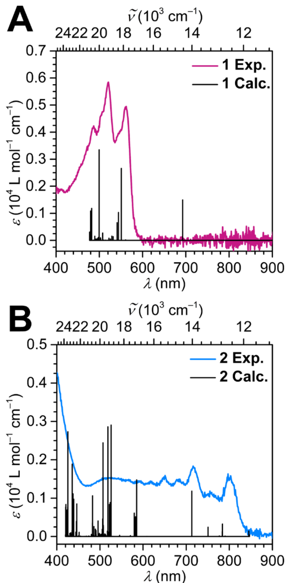
Fig. 5 UV-vis spectra of (A) [(\text{Cp}^*_2\text{Dy})_2(\mu\text{-tan})] (1) (pink line), and of (B) [(\text{Cp}^*_2\text{Dy})_2(\mu\text{-tan})][\text{BARF}_{20}] (2) (blue line), recorded at 32 \mu\text{mol L}^{-1} (1) and 140 \mu\text{mol L}^{-1} (2) concentrations in DCM at room temperature. Black vertical lines represent calculated TD-DFT transitions.
