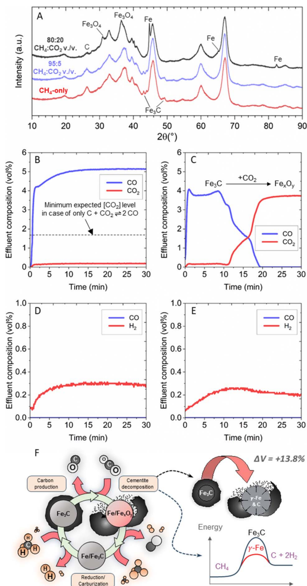
Fig. 3 Mechanism for the enhanced catalytic activity in OMP. (A) XRD spectra of 5 wt% Fe/ \theta - \text{Al}_2\text{O}_3 catalysts tested under methane-only, 95 : 5 \text{CH}_4 : \text{CO}_2 vol./vol. and 80 : 20 \text{CH}_4 : \text{CO}_2 vol./vol. feed. (B) \text{Fe}_3\text{C} and C mixture tested under a 95 : 5 Ar : \text{CO}_2 vol./vol. feed (C) \text{Fe}_3\text{C} tested under a 95 : 5 Ar : \text{CO}_2 vol./vol. feed. (D) \text{Fe}_3\text{C} and C mixture tested under a 99.1 : 0.9 Ar : \text{H}_2\text{O} vol./vol. feed. (E) \text{Fe}_3\text{C} tested under a 99.1 : 0.9 Ar : \text{H}_2\text{O} vol./vol. feed. (F) Graphical visualization of in situ cyclic formation-decomposition of cementite.
