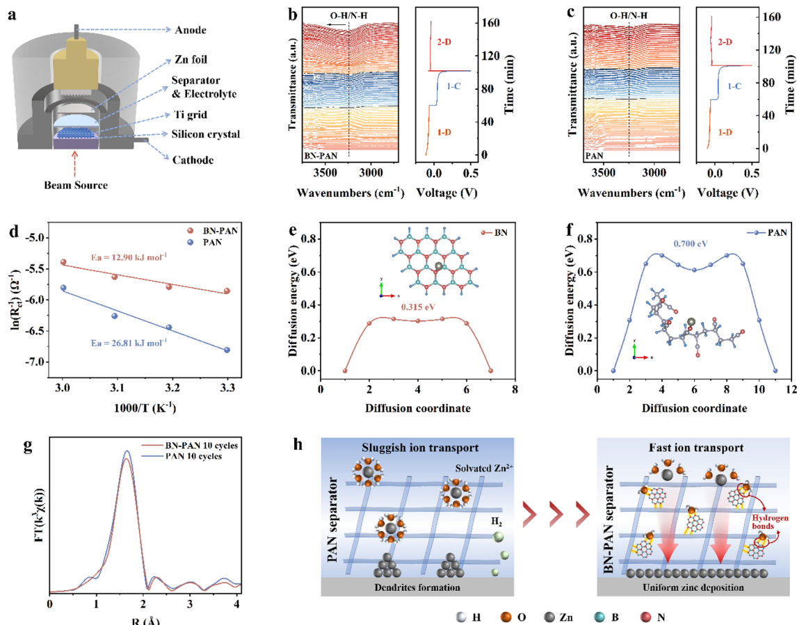
Fig. 2 Zn^{2+} transport mechanism of BN-PAN and PAN separators. (a) Schematic diagram of the device for the in situ FTIR test. In situ FTIR spectroscopy of Zn//Ti cells with the (b) BN-PAN separator and (c) PAN separator. (d) The comparison of activation energies of BN-PAN and PAN separators. The migration energy barrier of Zn^{2+} on (e) BN and (f) PAN. (g) Fourier-transformed Zn K-edge EXAFS spectra of BN-PAN and PAN separators after 10 cycles. (h) Schematic illustration of the Zn^{2+} transport mechanism with BN-PAN and PAN separators.
