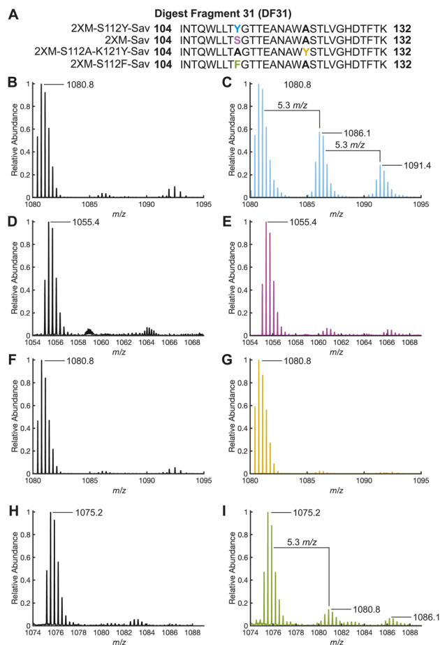
Fig. 4 (A) Digest fragment 31 sequences of variant 1, 2, 3 and 4. ESI-TOF positive-ion mode mass spectra [DF31] 3+ resulting from tryptic digests: 1 (B) before and (C) after the addition of 10 equivalents of H 2 O 2 and incubation for 1 hour. 2 (D) before and (E) after the addition of 10 equivalents of H 2 O 2 and incubation for 1 hour. 3 (F) before and (G) after the addition of 10 equivalents of H 2 O 2 and incubation for 1 hour. 4 (H) before and (I) after the addition of 10 equivalents of H 2 O 2 and incubation for 1 hour. Mass spectra were produced from the integration of LC peaks containing both unoxidized and oxidized DF31 (retention time: 2.85–3.10 min, Fig. S18–S20 and S27†).
