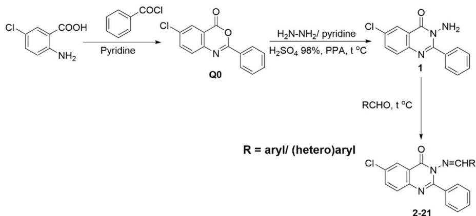
Scheme 1 Synthesis of 3-methylenamino-4(3 H )-quinazolinone derivatives (PPA: polyphosphoric acid).
