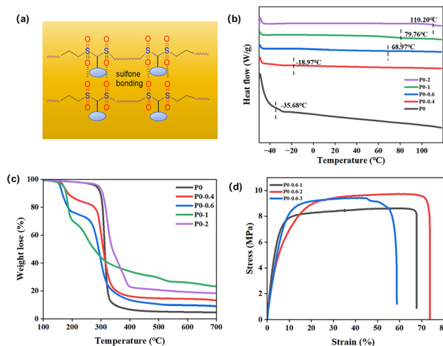
Fig. 3 (a) Schematic illustration of sulfone–sulfone interactions between the oxidized polydithioacetals; (b) DSC and (c) TGA analyses of P0 and the oxidized polymer products; and (d) tensile test results of polymers P0-0.6.
