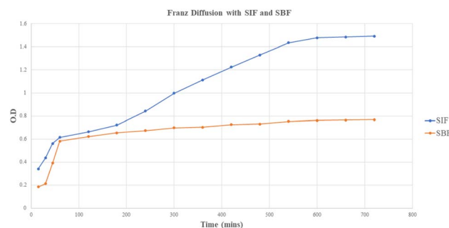
Fig. 6 Release profile of the core-shell nano-emulsion (MQ/GNE-GNP) in simulated intestine fluid (SIF) and simulated body fluid (SBF).
