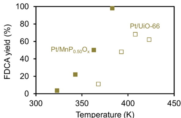
Fig. 4 Effect of reaction temperature on FDCA yield with a Pt/UIO-66 catalyst ( \square ) 74 and a Pt/MnP 0.50 O x catalyst ( \blacksquare ). 58 Reaction conditions for Pt/UIO-66 catalyst: HMF : Pt 200 : 1 molar ratio, P_{O_2} = 0.5 MPa, t = 14 h 74 and for Pt/MnP 0.50 O x catalyst: HMF : Pt 100 : 1 molar ratio, P_{O_2} = 1 MPa, t = 24 h. 58
