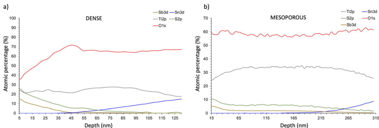
Fig. 10 XPS profiles for (a) glass-FTO/c-TiO 2 / \text{Sb}_2\text{S}_3 and (b) glass-FTO/c-TiO 2 /mp-TiO 2 / \text{Sb}_2\text{S}_3 samples.
