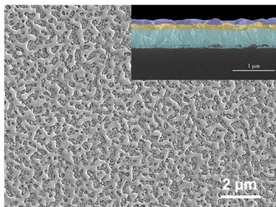
Fig. 9 SEM micrographs in top-view and cross-section (inset) of glass/FTO/c-TiO 2 /mp-TiO 2 / \text{Sb}_2\text{S}_3 sample. The following color code is used to label the consecutive layers: FTO glass (turquoise), c-TiO 2 and mp-TiO 2 (yellow) infiltrated by \text{Sb}_2\text{S}_3 , and overlayer of \text{Sb}_2\text{S}_3 (purple).
