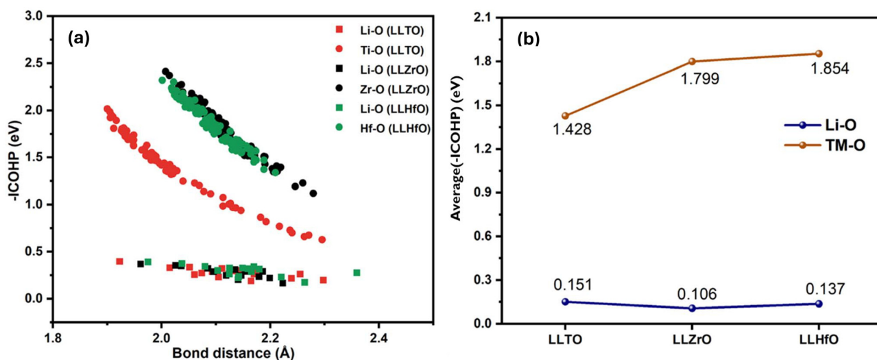
Fig. 3 (a) The comparative –ICOHP for the studied compositions for the Li@TS configurations. (b) The average –ICOHP of the diffusing \text{Li}^+ in the studied compositions for the Li@TS configurations. –ICOHP refers to the negative integrated Crystal Orbital Hamilton Population, used to evaluate bond strength between the diffusing \text{Li}^+ and surrounding atoms at the transition state (TS).
