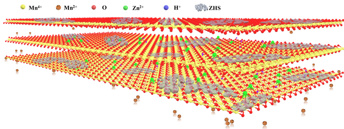
Fig. 1 With conflicting electrochemical reaction mechanisms in aqueous Zn–MnO 2 batteries, possible proposed storage mechanisms include Mn electrodedissolution–deposition, H + and/or Zn 2+ intercalation–deintercalation and ZHS (Zn 4 (OH) 6 SO 4 ·nH 2 O) deposition–dissolution are depicted in δ-MnO 2 , a layered phase, from a pool of available MnO 2 polymorphs.
