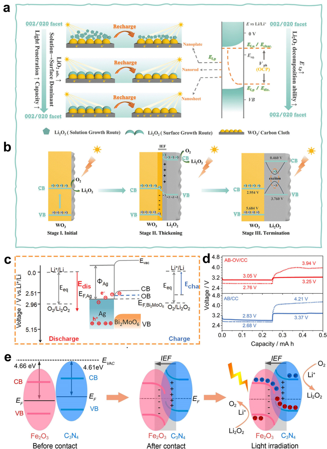
Fig. 15 (a) Facet-controlled \text{Li}_2\text{O}_2 growth pathways and the photocatalytic activity of \text{WO}_3 in photo-assisted Li-O 2 batteries. (b) Proposed mechanism of the photo-assisted discharge process, consisting of three distinct stages. 175 (c) Reaction mechanism of the AB-OV/CC photo-cathode in photo-assisted Li-O 2 batteries. (d) Discharge/charge profiles of AB-OV/CC and AB/CC photo-cathodes at a current density of 50 mA g -1 under illuminated (solid lines) and dark (dashed lines) conditions. 176 (e) Schematic illustration of directional charge transfer induced by the internal electric field at the \text{Fe}_2\text{O}_3/\text{C}_3\text{N}_4 interface. 177
