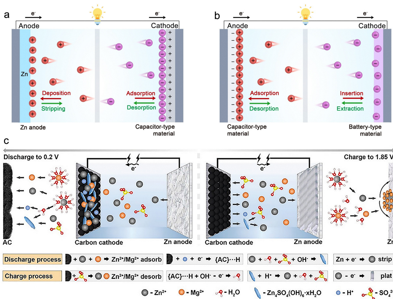
Fig. 19 Schematic illustrations of energy storage mechanisms in ZIHs: (a) a configuration comprising a capacitive cathode (based on electric double-layer capacitance or pseudocapacitance) coupled with a zinc deposition/stripping anode. (b) An alternative design employing a battery-type cathode (involving \text{Zn}^{2+} intercalation/deintercalation) paired with a capacitive anode (EDLC or pseudocapacitive behavior). (c) Schematic of AC||ZnMg-0.1||Zn energy storage devices. Reproduced with permission from ref. 346. Copyright 2021, Wiley.
