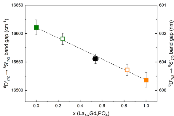
Fig. 7 Cm III excitation peak maxima (band gap energy) as a function of Gd III substitution (x) in La 1-x Gd x PO 4 monazite solid solutions. Adapted with permission from ref. 51. Copyright 2018 American Chemical Society.
