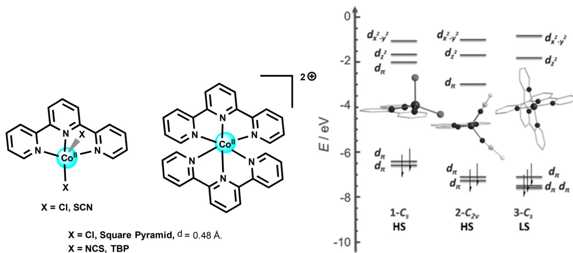
Fig. 12 Schematic representation of complexes 8a–8c (left) 77 and energy-level diagram depicting selected \beta -spin frontier molecular orbitals of 8a, 8b, and 8c (right), adapted/reproduced from ref. 77 with permission from Wiley, 77 copyright 2013.
