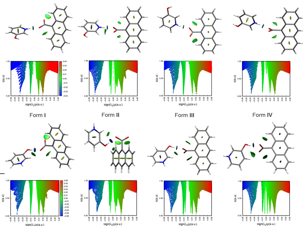
Fig. 4 Gradient isosurfaces of reduced density gradient, RDG in the area of O–H...O (-) and N (+) –H...O (-) hydrogen bonds identified in all four polymorphs supplied by fingerprint plots of the reduced density gradient (RDG) vs. the electron density multiplied by the sign of the second Hessian eigenvalue. Gradient surfaces are plotted at 0.1 au level. Full QTAIM characteristics of the bond critical points is given in Table 1.
