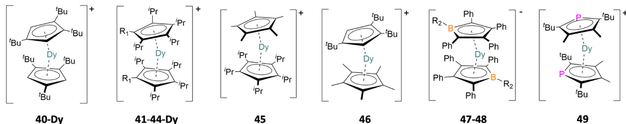
Fig. 6 Examples of the pseudo-linear dysprosocenium ions from [Dy(Cp ttt ) 2 ][B(C 6 F 5 ) 4 ] ( 40-Dy ), [Dy(Cp iPr ) 2 ][B(C 6 F 5 ) 4 ] ( 41 , R 1 = H), [Dy(Cp iPr Me) 2 ][B(C 6 F 5 ) 4 ] ( 42 , R 1 = Me), [Dy(Cp iPr Et) 2 ][B(C 6 F 5 ) 4 ] ( 43 , R 1 = Et), [Dy(Cp iPr ) 2 ][B(C 6 F 5 ) 4 ] ( 44-Dy , R 1 = iPr), [Dy(Cp iPr )(Cp*)][B(C 6 F 5 ) 4 ] ( 45 ), [Dy(Cp ttt )(Cp*)][Al(OC(CF 3 ) 3 ) 4 ] ( 46 ), [K(18-crown-6)(THF) 2 ][Dy(BC 4 Ph 5 ) 2 ] ( 47 , R 2 = Ph), [K(2.2.2)][Dy(BC 4 Ph 4 Pip) 2 ] ( 48 , R 2 = NC 5 H 10 ) and [Dy(PCl 4 tBu Me 2 ) 2 ][Al(OC(CF 3 ) 3 ) 4 ] ( 49 ). 59–62,67–69
