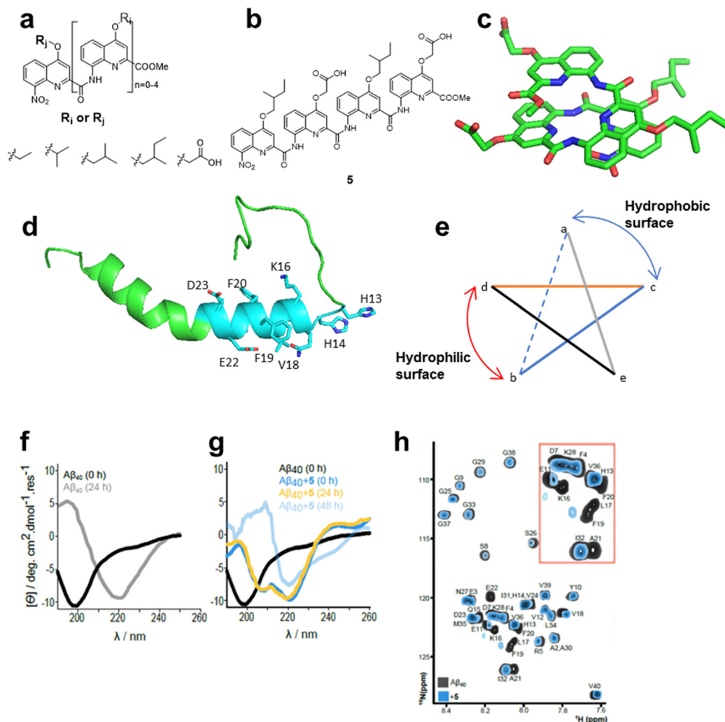
Fig. 2 (a) Generic scheme for the chemical structures of quinoline foldamers. (b) Chemical structure of quinoline 5. (c) 3D model of quinoline 5. 77 (d) The partially folded NMR structure of A \beta_{40} used to highlight the binding region of quinoline 5 (turquoise labeled). (e) Top view of the oligoquinoline foldamer. (f) Circular dichroism of 20 \mu\text{M} A \beta_{40} at 0 h and 24 h. (g) Circular dichroism of A \beta_{40} at multiple time points in the presence of an equimolar amount of 5. (h) Overlay of the ^1\text{H} - ^{15}\text{N} HSQC NMR spectrum of 60 \mu\text{M} A \beta_{40} in the absence and presence of 5 ( ^{15}\text{N} -A \beta_{40} : 5 = 1 : 2).
