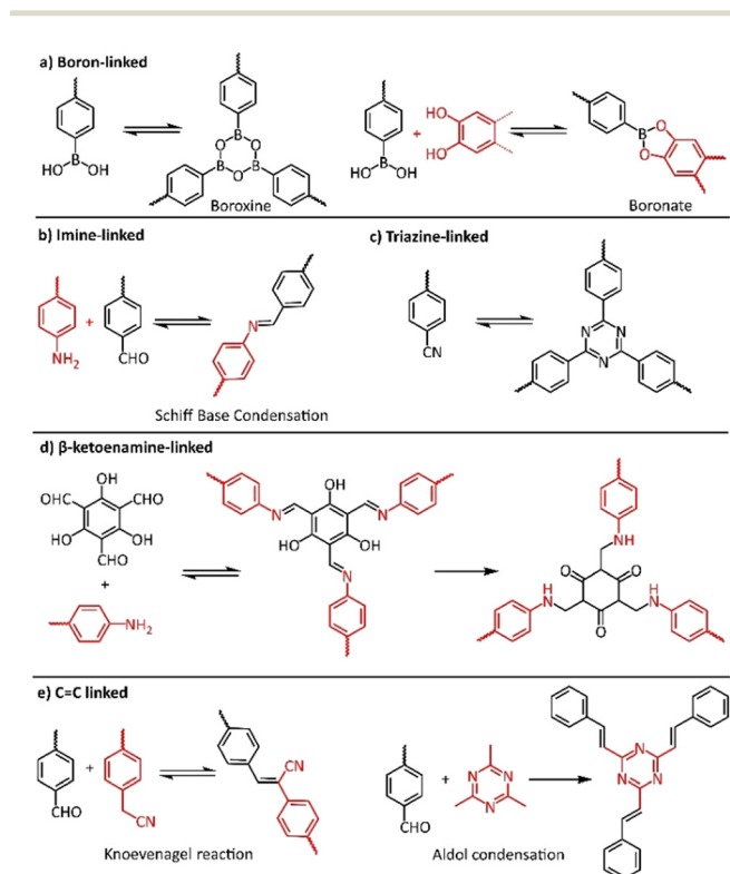
Fig. 3 Typical covalent linkage reactions for COF synthesis.
