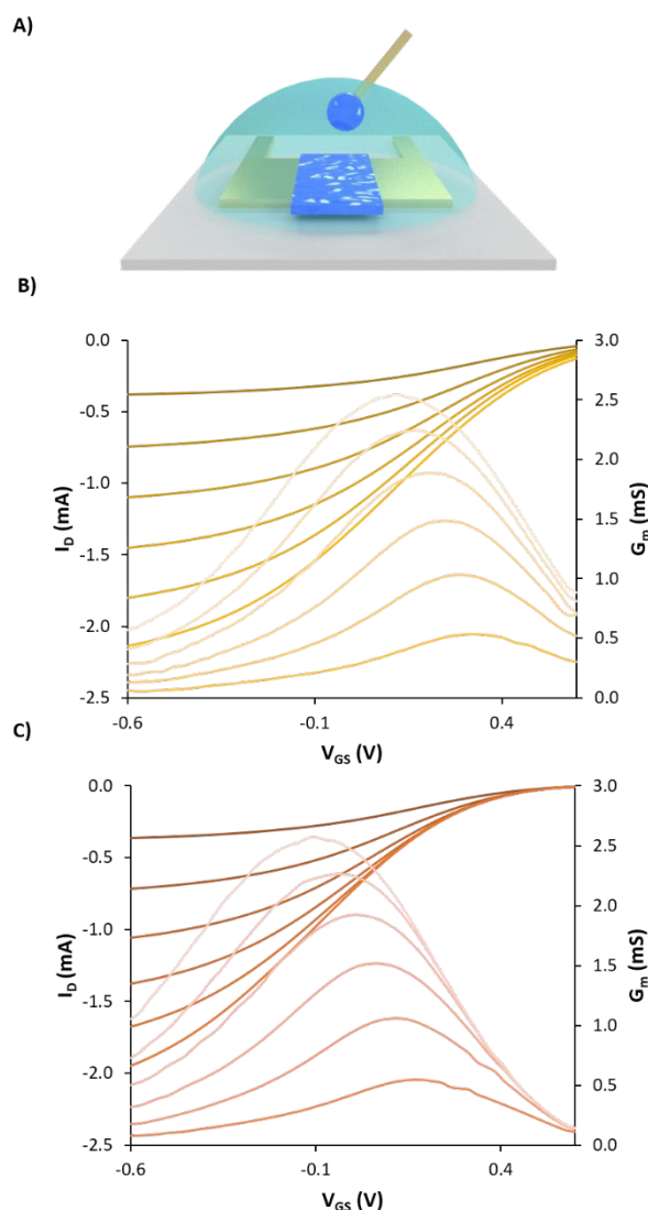
Figure 6. A) Schematic representation of an OECT; PEDOT:PSS is deposited on the channel between the drain and source while the electrogelated Ag/Cu/PEDOT:PSS-co-PSMA is used as gate electrode. Transfer-characteristics and transconductance curves at varying drain voltages from 0 to -0.6 V of OECTs with a channel of L = 600\mu\text{m} , W = 70 \mu\text{m} , of B) bare gold gate and C) Ag/Cu/PEDOT:PSS-co-PSMA (C) gate. For all cases, R = 2\text{mm} and the V_D is set from -0.1 to -0.6 V with an interval of 0.1 V
