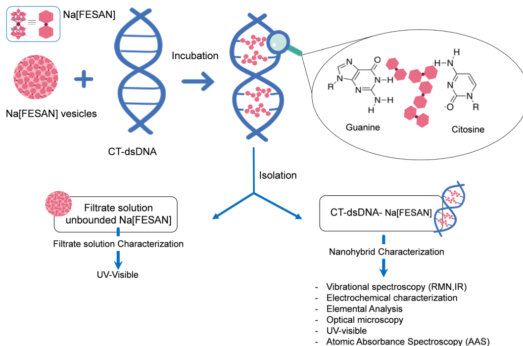
Fig. 3 Schematic representation of the preparation, isolation and characterization of the nanohybrid CT-dsDNA-Na[o-FESAN]; emphasizing the amplification of intercalation between amphiphilic small [\text{o-FESAN}]^- molecules and the double strand of DNA molecules with the double strand of DNA.
