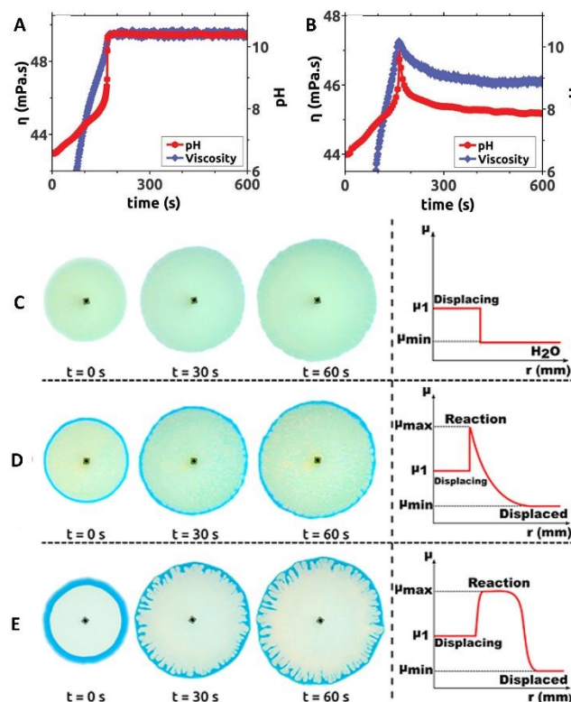
Figure 6. Temporal evolution of pH and viscosity in (A) MGS and (B) MGS-GL systems containing poly(acrylic acid) PAA. Initial concentrations: sulfite 68.4 mM, formaldehyde 65.3 mM, PAA 0.4386 wt%. In (B) the initial concentration of GL is 7 mM. For the viscosity measurement, the shear rate and temperature were fixed respectively at 500 \text{s}^{-1} and 23°C, respectively. Image reproduced with permission from ref. 36 . (C-E) Solution displacement experiments performed in a Hele-Shaw cell. The initial formaldehyde concentration in the displaced solution is (C) 0 mM, (D) 49.6 mM, (E) 750 mM. In (E) the appearance of viscous fingering instability is clearly visible. The other initial concentrations are, in all cases, sulfite 68.4 mM, PAA 0.4386 wt%, bromothymol blue (yellow for pH < 6, green for pH ~ 6-7, blue for pH > 7) 0.021 wt%. The injection speed of the displacing solution was 7 \text{mL min}^{-1} . In the schematic profiles on the right, \mu_{\text{min}} , \mu_{\text{max}} and \mu_1 indicate respectively the minimum, maximum, and displacing solution viscosity values. Adapted with permission from ref. 37 . Copyright 2019 American Chemical Society.
