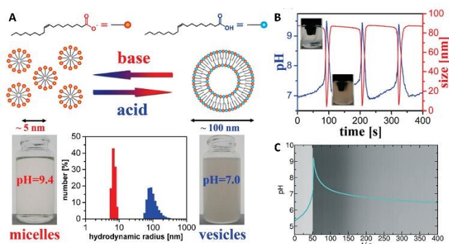
Figure 4. (A) Schematic representation of deprotonated (orange) and protonated (blue) oleic acid molecules, along with their self-assembly structures, respectively micelles (transparent solution, basic pH) and vesicles (turbid suspension, acidic pH). The difference in size is confirmed by hydrodynamic radius measurements. (B) Cyclic, oscillatory vesicle-to-micelle transition obtained using a MGS-GL-oleic acid system in a CSTR, visualized through pH and hydrodynamic size measurements. The reactor was continuously fed by a constant (1.52 mL min -1 in each channel) flow of two solutions, one containing 10 mM sulfite, 100 mM bisulfite and 1% m/m oleic acid, the other containing 200 mM formaldehyde and 13.4 mM GL. The reaction volume was kept fixed (10 mL) by removing reaction products at a constant rate (3.04 mL min -1 ). Adapted with permission from ref. 34 . Copyright 2010 American Chemical Society. (C) Evolution over time of pH (blue line) and solution turbidity (background) in a batch MGS-GL system containing 1.25 mM oleic acid (initial concentrations: 5 mM sulfite, 50 mM bisulfite, 200 mM MG, 10 mM GL). Image reproduced from ref. 31
