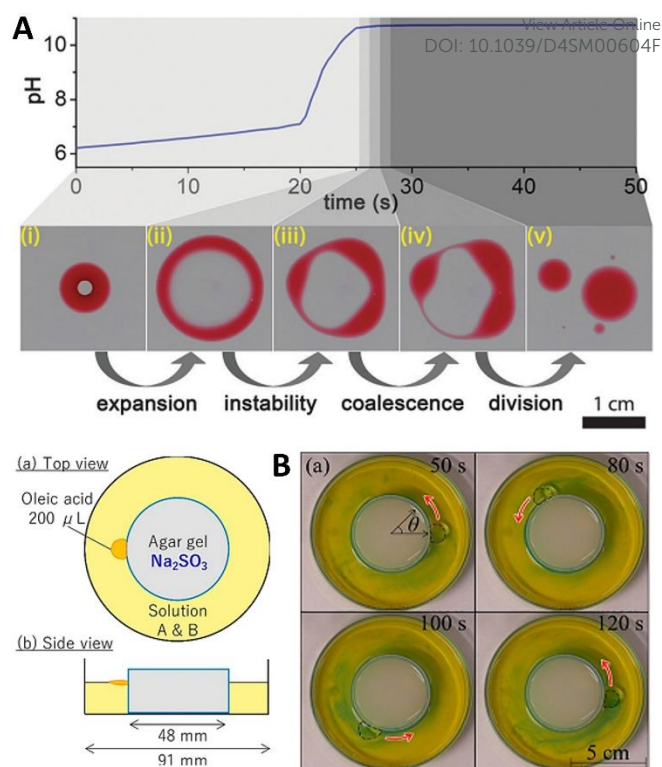
Figure 9. (A) Self-division of a compartmentalized oil droplet (2-hexyldecanoic acid in paraffin, red) containing a MGS clock mixture (colorless; initial concentrations: 10 mM sulfite, 100 mM bisulfite, 200 mM formaldehyde), floating on a water surface. When the pH inside inside the compartment becomes basic, the deprotonation of the fatty acid molecules results in a surface tension change leading to the destabilization and expansion of the droplet into a ring-like structure. The latter undergoes Plateau-Rayleigh instability and divides into smaller droplets. Image reproduced from ref. 41 . (B) Schematic representation and experimental pictures of the setup used by Shioi and coworkers to obtain the autonomous movement of an oleic acid droplet around a sulfite-containing agarose gel, sustained by the MGS-GL system ("solution A & B") with initial concentrations of 1.25 mM sulfite, 208 mM bisulfite, 500 mM formaldehyde, 3.40 mM GL, and a small amount of bromothymol blue for visualizing local pH changes (blue pH > 7.6, yellow pH < 6.0). Images reproduced from ref. 42
