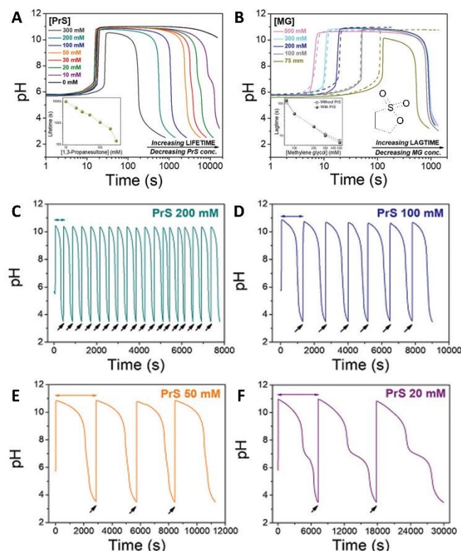
Figure 3. (A,B) Effect of the initial concentration of (A) PrS, (B) MG on the pH-time evolution profile, as well as on t_{\text{clock}} and
