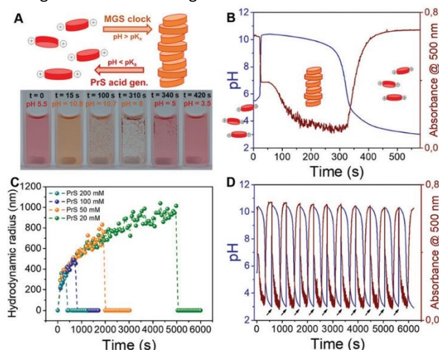
Figure 5. Autonomous self-assembly/disassembly cycle of a pH-responsive perylene diimide controlled by the MGS-PrS system (initial concentrations: sulfite 5 mM, bisulfite 50 mM, MG 200 mM, PrS 100 mM). (A) Schematic representation and experimental photographic sequence. (B,C) The transient formation of aggregates in correspondence of the pH increase to basic (MGS clock) and their subsequent dissolution when the pH becomes acidic (PrS hydrolysis) can be visualized (B) by measuring pH while acquiring absorption spectra over time, or (C) by measuring the evolution of hydrodynamic radius by dynamic light scattering (DLS) over time. As shown in (D), cycles of self-(dis)assembly can be repeated with remarkable stability in semi-batch conditions by the external addition of a base (NaOH aqueous solution, black arrows). The images are reproduced from ref. 32
