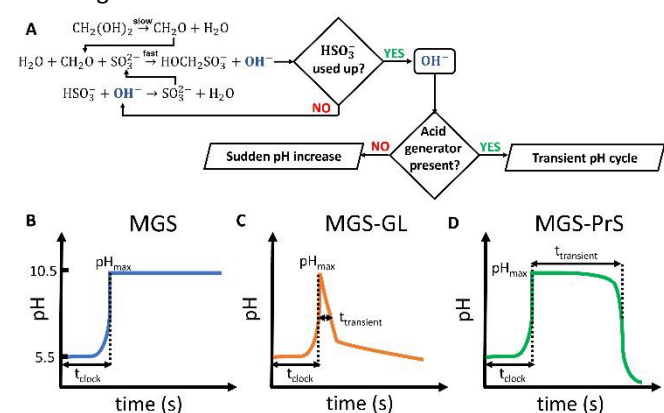
Figure 1. (A) Main reactions involved in the methylene glycol-sulfite (MGS) pH-clock, together with (B-D) characteristic pH-time profiles obtained without and with the addition of slow
