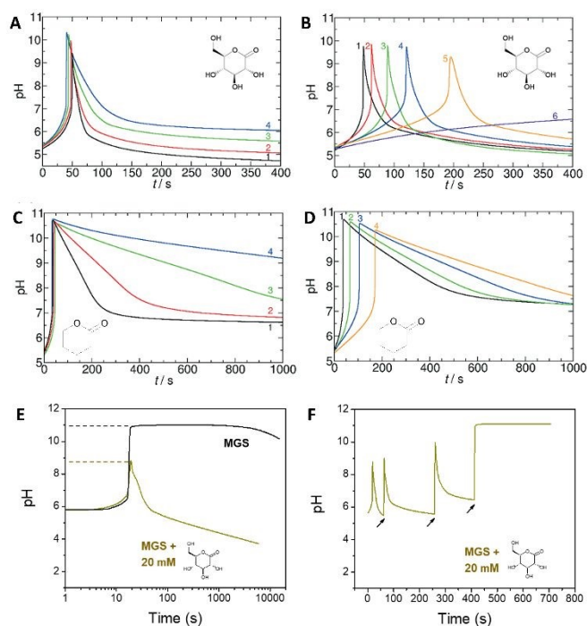
Figure 2. (A,B) Effect of the initial concentration of (A) GL, (B) MG on the pH-time evolution profile, as well as on t_{\text{clock}} and t_{\text{transient}} for the MGS-GL system. The initial concentration of sulfite and bisulfite is respectively 5 mM and 50 mM. In (A) the initial concentration of MG is 200 mM, while the initial concentration of GL varies in the order 20/10/5/4 mM (curves 1-4). In (B) the initial concentration of GL is 10 mM, while the initial concentration of MG varies in the order 200/175/150/125/112.5/100 mM (curves 1-6). (C,D) Same as (A,B) but for the MGS-VL system. In (D) the initial MG concentrations are 200/150/125/112.5 mM (curves 1-4). The molecular structures of GL and VL are shown as insets. (E) Comparison of the pH-time profile for the MGS clock (initial concentrations: sulfite 5 mM, bisulfite 50 mM, MG 200 mM) without and with the addition of 20 mM GL. In (F), in the attempt to make semi-batch pH cycles, the pH is brought back to alkaline by the external addition (black arrows) of a 2 M sodium hydroxide solution. The first two additions are of 30 \mu\text{L} and the third one of 40 \mu\text{L} , corresponding to a total of 20 mM NaOH. Already after the first cycle the time required to reach the same final pH increases dramatically, while after the third cycle the GL is completely hydrolyzed (pH plateau) preventing the generation of further cycles. The images in (A-D) are reproduced from ref. 31 , those in (E,F) are reproduced from ref. 32
