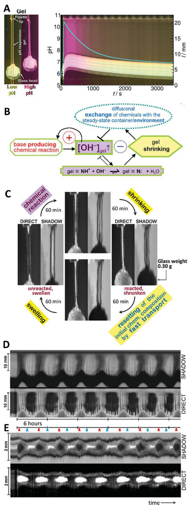
Figure 10. (A) Space-time plot of gel length and the synchronous pH-change (blue line) in a batch MGS-VL system (initial concentrations: sulfite 5 mM, bisulfite 50 mM, MG 112.5 mM,
