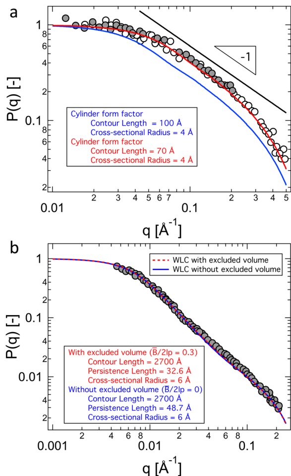
Fig. 29 Form factor of TMAPSS in (a) salt-free aqueous solution (grey circles c = 0.2 M, white circles c = 0.1 M, c^* \approx 1 M based on Fig. 11) and (b) 0.19 M TMAPSS solution. Lines are fit to the cylinder form factor for (a) and to the worm-like chain form factor with and without excluded volume for (b). The fit parameters are indicated in the legend. The black line in the top panel represents the power law of -1 . Cylinder form factors and WLC with excluded volume are calculated using SASView v 5.0.6. Data are from ref. 125 and 615.
