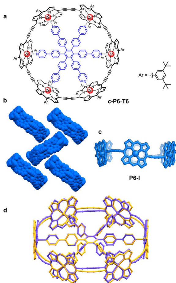
Fig. 1 (a) Drawing of a six-porphyrin nanoring with the template marked in blue, Ar = 3,5-di- tert -butylphenyl. (b) Fragment of the crystal structure of the previously reported, orthorhombic ( P ccc) polymorph P6-I (CCDC: 860774). 6 (c) View of the molecular conformation of the nanoring in P6-I . Hydrogen atoms, template and aryl groups in (b) and (c) are omitted for clarity. (d) Comparison of the molecular geometry of c-P6·T6 from the published crystal structure of polymorph P6-I (purple) 6 and the gas-phase geometry from DFT calculations (BLYP35/6-31G*, yellow). 16
