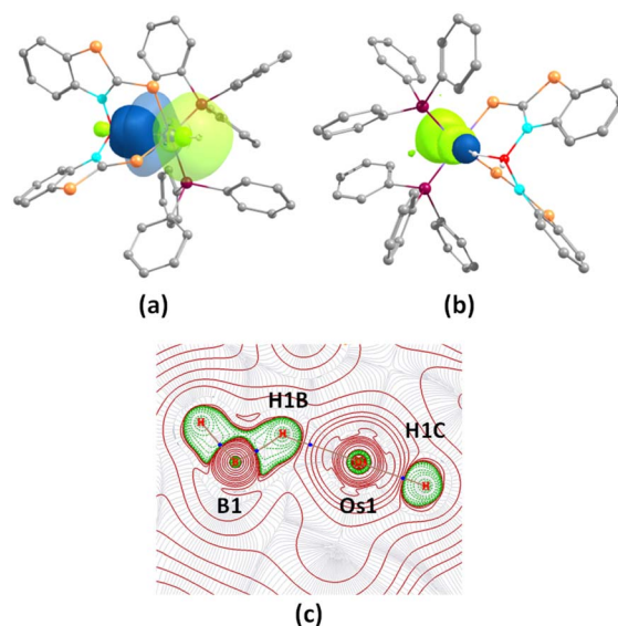
Fig. 6 (a) Donor–acceptor interaction between \sigma(\text{B–H}) and the Os center in 4a ; (b) Os–H bonding interaction in 4a (isovalue 0.004 [ e bohr ^{-3/2} ]); (c) contour-line diagram of the Laplacian of the electron density along Os–H–B planes in 4a .
