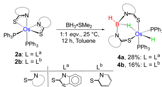
Scheme 2 B–H activation by Os(II)- N,S -chelated complexes, 2a–b .
