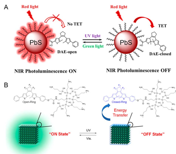
Fig. 3 (A) Photoswitchable photoluminescence of diarylethene-bound PbS QDs. 54 Adapted with permission from ref. 50. Copyright 2022 American Chemical Society. (B) Photoswitchable perovskite lead halide QDs coated by triethoxysilane-modified diarylethene. 62 Adapted with permission from ref. 57. Copyright 2020 American Chemical Society.
