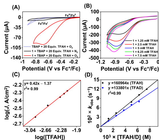
Fig. 6 (A) The cyclic voltammogram of 1 (0.5 mM) was measured in an oxygen-saturated acetonitrile solution containing 10 mM of TFAH and 50 mM nBu 4 NPF 6 as the supporting electrolyte at 25 °C (scan rate 0.1 V s −1 ). The black trace was taken in the absence of oxygen. The dotted blue trace was taken in the absence of 1 under oxygen. (B) Cyclic voltammogram of 1 (0.5 mM) measured at different concentrations of TFAH (1.25–7.5 mM) in oxygen-saturated acetonitrile with a scan rate of 6 V s −1 at 25 °C. (C) A plot of log( J , A cm −2 ) vs. log([TFAH]) for 1 (0.5 mM) in oxygen saturated acetonitrile containing 50 mM nBu 4 NPF 6 (scan rate 6 V s −1 ). (D) A plot of k obs vs. [TFAH/D] at a fixed concentration of 1 (0.5 mM) and O 2 (6.0 mM) at 25 °C.
