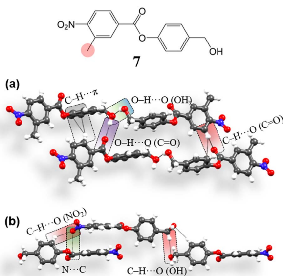
Fig. 9 (a and b) Intermolecular interactions involved in the crystal packing of 7 .
