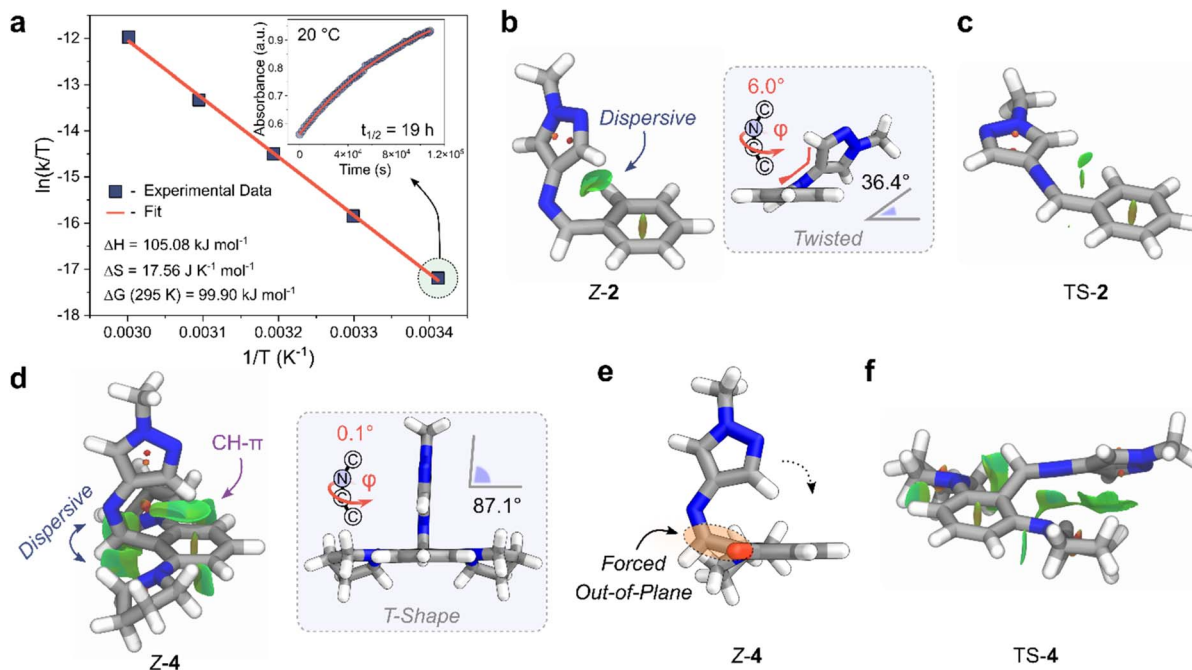
Fig. 5 (a) Eyring plot of the longest-lived Z-AIP, 4 . (inset) Rate of thermal reversion of the Z-to-E isomer at 20^\circ\text{C} . (b) Geometry-optimized Z-2 highlighting green NCI surfaces between the pyrazole and phenyl rings. (inset) Display of the twisted geometry. (c) Geometry-optimized TS-2 with NCI surfaces displayed. (d) Geometry-optimized Z-4 showing large NCI interactions between the imine and the ortho -pyrrolidine units, as well as CH- \pi interactions between the CH of the pyrazole and the phenyl ring. (inset) View showing the T-Shape conformation. (e) Alternate view of Z-4; the pyrrolidine projecting out of the page is depicted as a red stub for clarity. (f) Geometry-optimized structure of TS-4 with NCI surfaces displayed.
