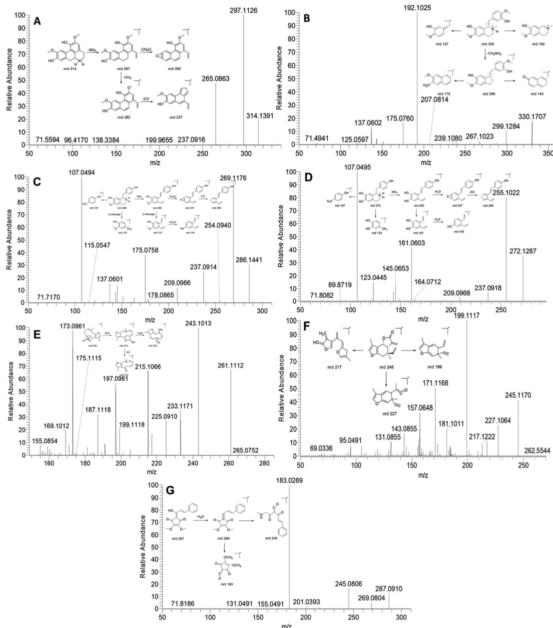
Fig. 1 MS/MS spectra and the proposed fragmentation pathway of norisoboldine (A), reticuline (B), coclaurine (C), higenamine (D), linderane (E), isolinderac lactone (F), and linderone (G).
