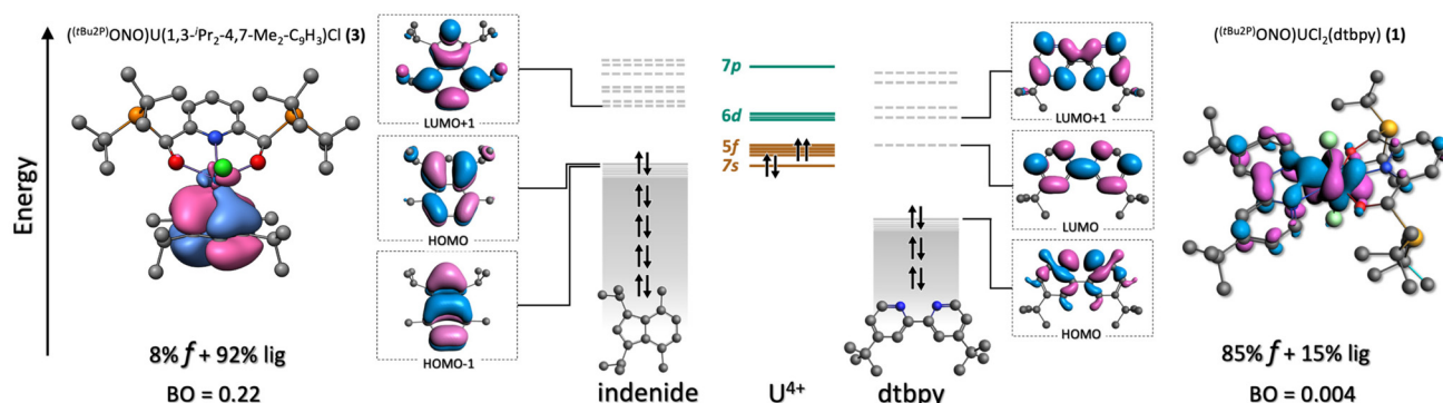
Fig. 6 Qualitative molecular orbital diagram of 1 and 3. The brown lines/blocks indicate occupied orbitals while the green lines correspond to empty orbitals. As observed, the LUMO and LUMO+1 of the dtbpy ligand are close in energy to the 5f manifold. In consequence, an interaction displaying a small degree of back-donation (depicted in the right side) takes place. In the case of 3, the energetics is different and no back-bonding is observed. However, focusing on the HOMO of the indenide ligand, it is noteworthy how the 5-member ring orbital symmetry has a better match with the 5f orbitals than that of the 6-member ring. This interaction forms the dative interaction depicted in the left side. Isovalue = 0.03.
