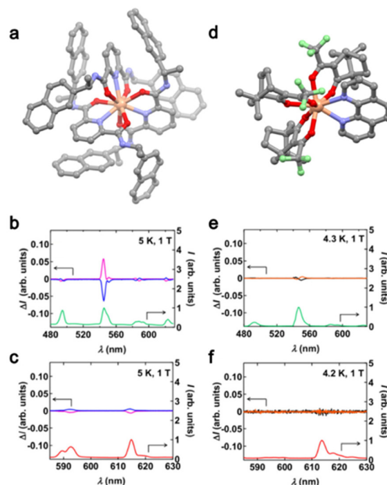
Fig. 1 (a) Molecular structure of (\text{S,S})2\text{-Tb} . Grey, C; red, O; blue, N and salmon, Tb. H atoms and \text{CF}_3\text{SO}_3^- anions are omitted for clarity. (b) Average luminescence spectrum of (\text{S,S})2\text{-Tb} (green line) and MChD spectra of (\text{S,S})2\text{-Tb} (pink line) and (\text{R,R})2\text{-Tb} (blue line). (c) Average luminescence spectrum of (\text{S,S})2\text{-Eu} (red line) and MChD spectra of (\text{S,S})2\text{-Eu} (pink line) and (\text{R,R})2\text{-Eu} (blue line). (d) Molecular structure of (d)3\text{-Tb} . Grey, C; red, O; blue, N; green, F and salmon, Tb. H atoms are omitted for clarity. (e) Average luminescence spectrum of (d)3\text{-Tb} (green line) and MChD spectra of (d)3\text{-Tb} (black line) and (l)3\text{-Tb} (orange line). (f) Average luminescence spectrum of (d)3\text{-Eu} (red line) and MChD spectra of (d)3\text{-Eu} (black line) and (l)3\text{-Eu} (orange line). Adapted with permission from ref. 12. Copyright 2019, American Physical Society.
