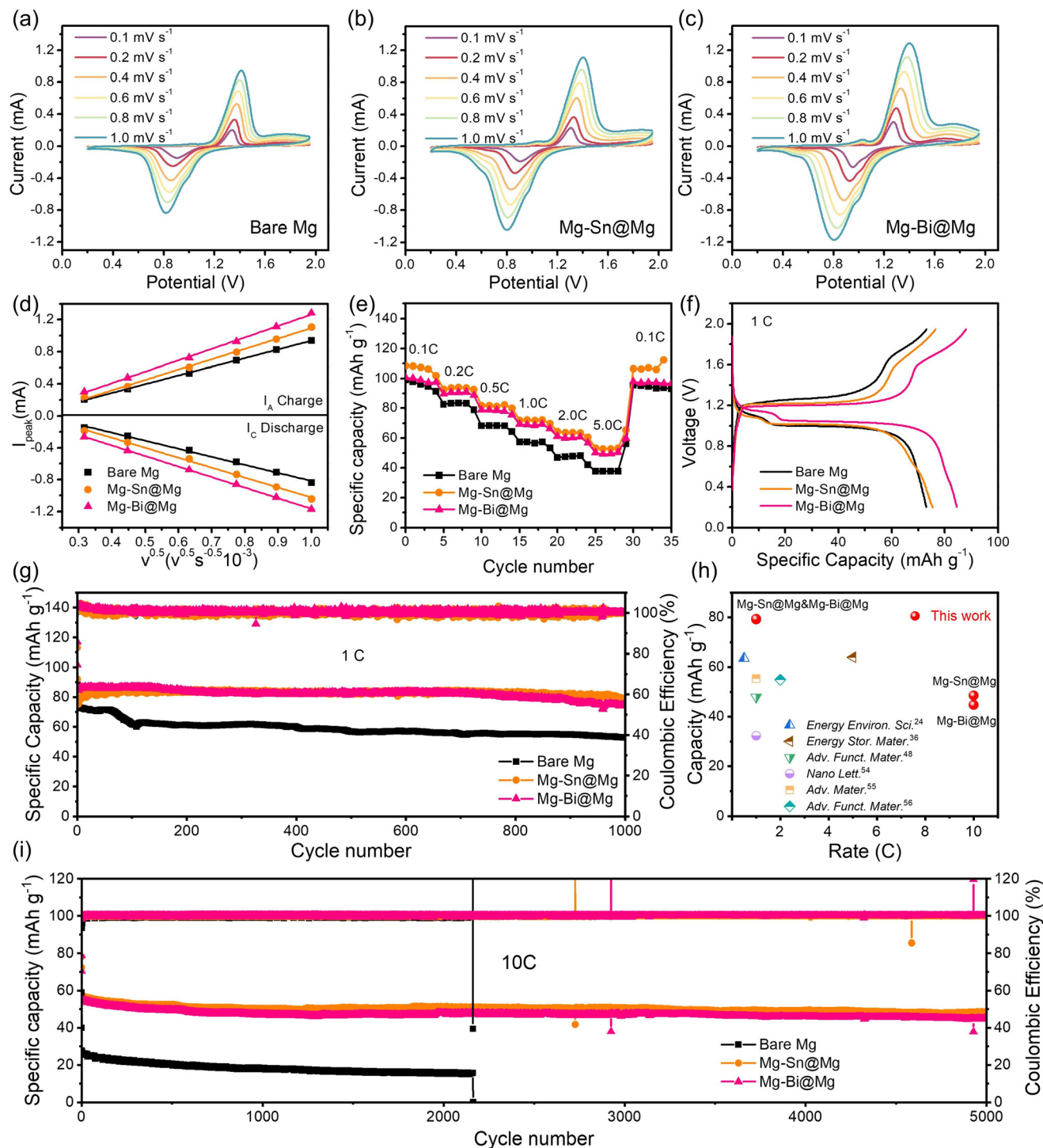
Fig. 6 CV curves of (a) \text{Mo}_6\text{S}_8 /bare Mg, (b) \text{Mo}_6\text{S}_8 /Mg-Sn@Mg and (c) \text{Mo}_6\text{S}_8 /Mg-Bi@Mg full cells at different scan rates from 0.1 to 1.0 \text{mV s}^{-1} in the voltage range of 0.2–1.95 V and (d) the square root of scan rate ( v^{0.5} ) of bare Mg, Mg-Sn@Mg and Mg-Bi@Mg full cells. (e) Rate performance of the \text{Mo}_6\text{S}_8 /bare Mg, \text{Mo}_6\text{S}_8 /Mg-Sn@Mg and \text{Mo}_6\text{S}_8 /Mg-Bi@Mg full cells. (f) The first charge–discharge profiles for \text{Mo}_6\text{S}_8 /bare Mg, \text{Mo}_6\text{S}_8 /Mg-Sn@Mg and \text{Mo}_6\text{S}_8 /Mg-Bi@Mg full cells at 1 C. (g) Cycling performance of the \text{Mo}_6\text{S}_8 /bare Mg, \text{Mo}_6\text{S}_8 /Mg-Sn@Mg and \text{Mo}_6\text{S}_8 /Mg-Bi@Mg full cells at 1 C. (h) The capacity and cycling stability performance of the \text{Mo}_6\text{S}_8 /Mg-Sn@Mg and \text{Mo}_6\text{S}_8 /Mg-Bi@Mg cells compared with those of previously reported \text{Mo}_6\text{S}_8 /Mg full cells. 26,38,55,61–63 (i) Cycling performance of \text{Mo}_6\text{S}_8 /bare Mg, \text{Mo}_6\text{S}_8 /Mg-Sn@Mg and \text{Mo}_6\text{S}_8 /Mg-Bi@Mg full cells at 10 C.
