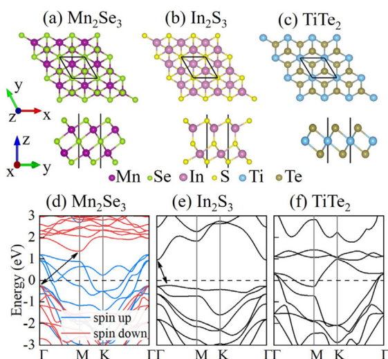
Fig. 1 The top and side views of the crystal structures of (a) \text{Mn}_2\text{Se}_3 , (b) \text{In}_2\text{S}_3 and (c) \text{TiTe}_2 monolayers. The band structures of (d) \text{Mn}_2\text{Se}_3 , (e) \text{In}_2\text{S}_3 and (f) \text{TiTe}_2 monolayers.
