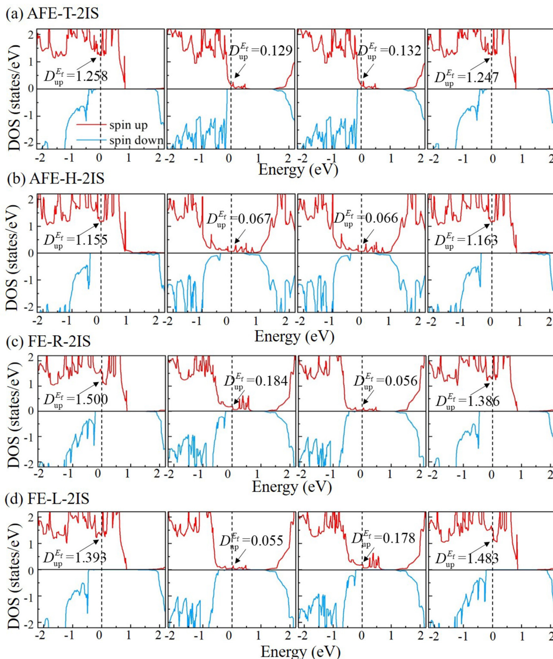
Fig. 5 The spin-dependent DOS of the Mn 2 Se 3 /bilayer-In 2 S 3 /Mn 2 Se 3 part in the MFTJ with (a) AFE-T-2IS, (b) AFE-H-2IS, (c) FE-R-2IS and (d) FE-L-2IS states. D_{up}^{E_f} represents the spin-up DOS value at the Fermi level.
