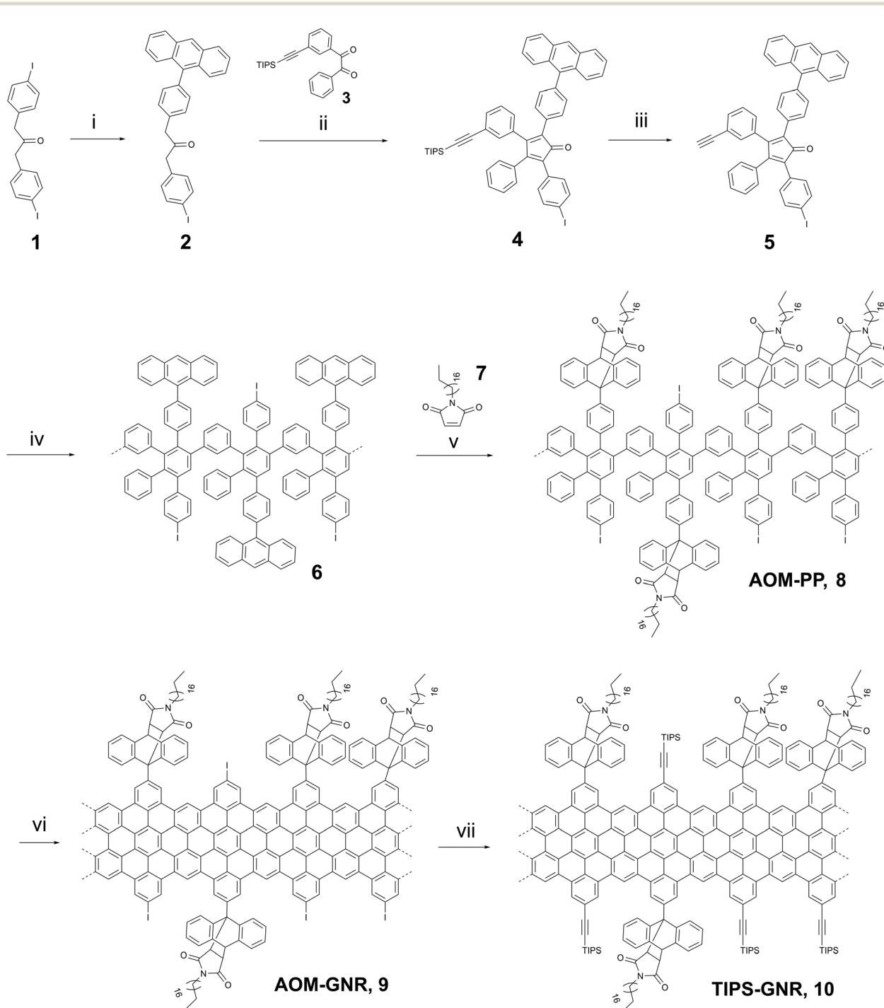
Scheme 1 Synthetic route of “clickable” GNRs 10 : (i) anthracene-9-yl-boronic acid, Pd(PPh 3 ) 4 , K 2 CO 3 , THF, 12 h, 60 °C, 47%, (ii) NBu 4 NOH, 1.5 h, 65 °C, t -BuOH, 79%, (iii) TBAF, RT, CH 2 Cl 2 , 20 min, 67%, (iv) Ph 2 O, 250 °C, 36 h, 79%, (v) o -Xylene, 36 h, 150 °C, 92%. (vi) FeCl 3 (2.76 × 10 -3 M), CH 2 Cl 2 /MeNO 2 , 72 h, RT, 92%, (vii) ethynyltriisopropylsilane, THF/NEt 3 , 72 h, RT, 86%.
