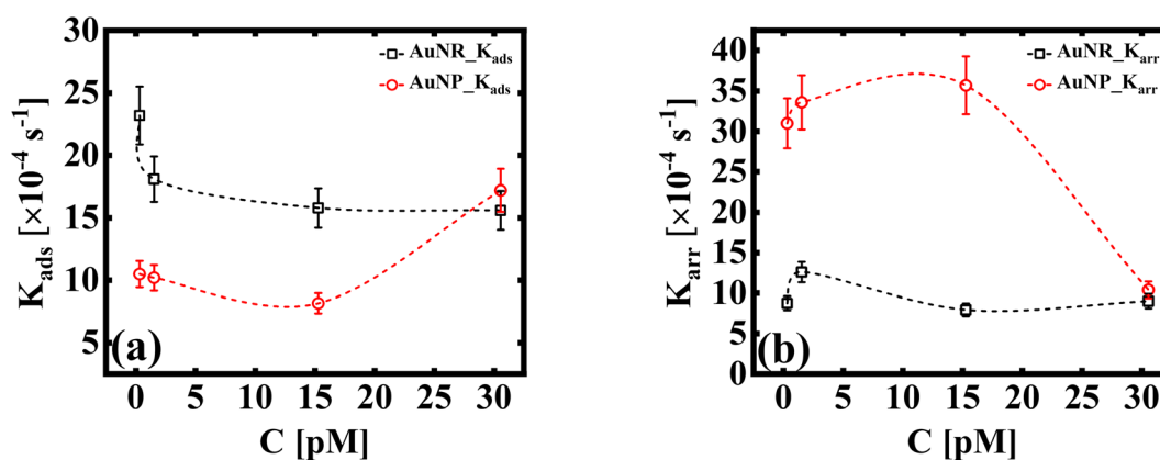
Fig. 4 (a) First order adsorption rate, K_{\text{ads}} , and (b) molecular rearrangement rate, K_{\text{arr}} , of adsorbed particles at the liquid/liquid interface (dashed lines as a guide to the eye). The estimates in (a and b) are obtained using the linear regression model given by eqn (5).
