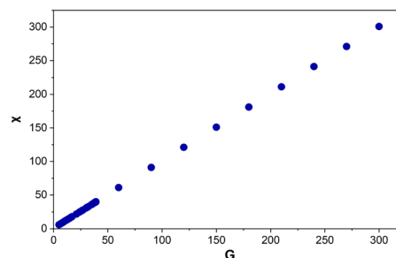
Fig. 9 Euler's characteristic ( \chi ) for Voronoi structures designed from 5–300 generating points ( G ). Each data point is an average of 125–800 Voronoi structures.
