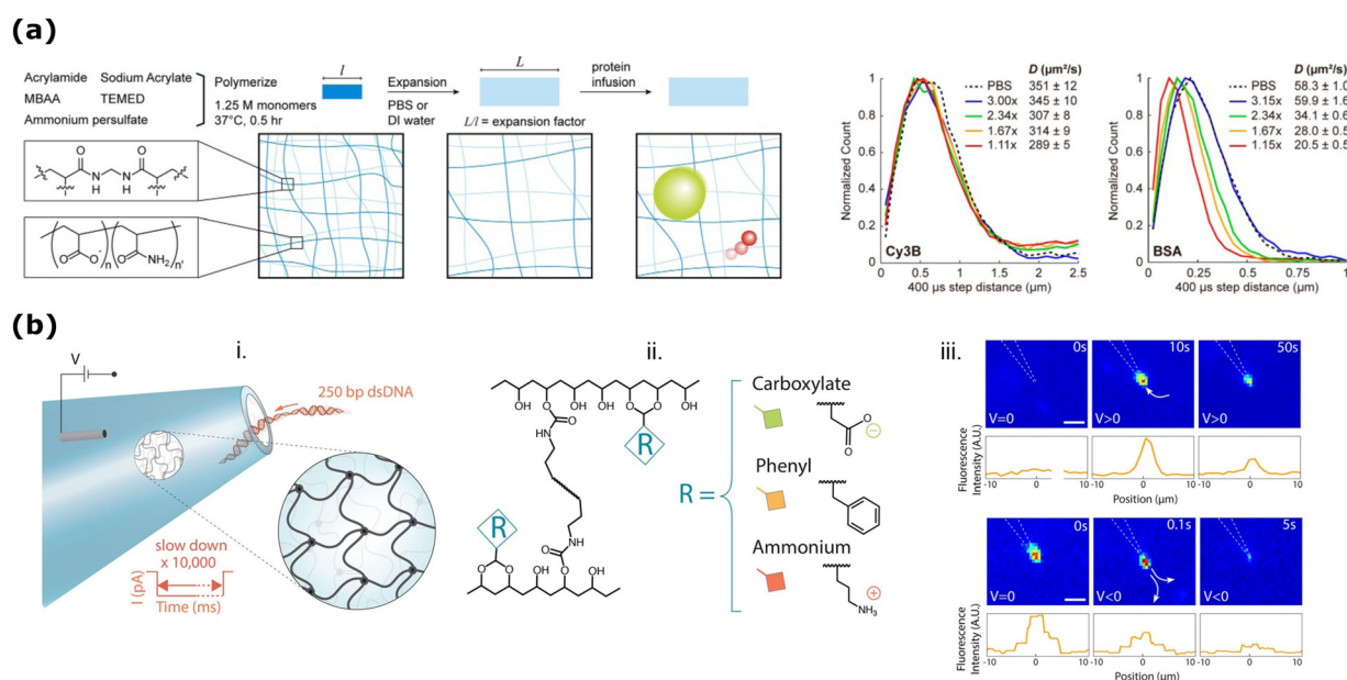
Fig. 10 (a) (Left) Schematic representation of hydrogel synthesis and of the diffusion process studied; (right) Normalized count distributions of the SMdM-measured 400 μs single-molecule displacements for Cy3B diffusing in PBS (dash line) and in hydrogels with different expansion factors (solid lines), with respective maximum likelihood estimation results shown in the legend. Adapted with permission from ref. 298 Copyright 2023, American Chemical Society. (b) (i) Schematic representation of the hydrogel functionalized nanopipette (HFN) sensor showing a 3D cross-linked nanoporous mesh at the tip of the nanopipette, (ii) simplified chemical structure of the photo-cross-linked PVA-based hydrogels, (iii) optical tracking of individual YOYO-1 labeled 10 kbp dsDNA molecules at the HFN tip (scale bars show 2 μm). Reprinted with permission from ref. 297 Copyright 2018, American Chemical Society.
