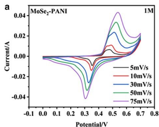
Figure 16. CV curves at different scanning rates [Reproduced from ref. 83, with permission from Springer, copyright 2023]
