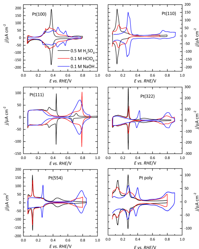
Fig. 1 Voltammetric profiles of the low index planes of Pt (Pt(100), Pt(110), and Pt(111)), two stepped surfaces, Pt(322) and Pt(554) containing (111) terraces and (100) and (110) steps, respectively, and a polycrystalline Pt electrode in different electrolytes. Electrodes were cooled down in a \text{H}_2/\text{Ar} atmosphere after flame annealing. Scan rate: 50 \text{ mV s}^{-1} .
