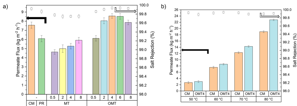
Fig. 6 Average total permeate flux and salt rejection of the prepared PVDF-clay membranes at a) 60^\circ\text{C} and at b) different feed temperatures for commercial PVDF and the OMT 4 wt% membranes. Columns: permeate flux ( \text{kg m}^{-2} \text{ h}^{-1} ), and square symbols \square : salt rejection (%). Error bars represent standard deviations from three samples.
