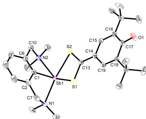
Fig. 6 Representation of the molecular structure of \{[NCN^{Me_4}]Sb(S_2C_6H_2-tBu_2-3,5-O-4)\} ( 13 ). H atoms and non-interacting pyridine molecules omitted for clarity. Ellipsoids at the 50% probability level. Selected distances (Å) and angles ( ^\circ ): Sb1–C1 = 2.1429(17), Sb1–N1 = 2.5492(15), Sb1–N2 = 2.6003(15), Sb1–S1 = 2.5505(5), Sb1–S2 = 2.5723(5), C17–O1 = 1.248(2), S1–C13 = 1.7369(17), S2–C13 = 1.7364(17), C13–C14 = 1.395(2), C14–C15 = 1.429(2), C14–C19 = 1.431(2), C15–C16 = 1.358(2), C16–C17 = 1.474(2), C17–C18 = 1.475(2), C18–C19 = 1.355(2); C1–Sb1–N1 = 72.36(6), C1–Sb1–N2 = 71.69(6), C1–Sb1–S1 = 96.31(5), C1–Sb1–S2 = 96.96(5), N1–Sb1–N2 = 126.95(5), N1–Sb1–S1 = 78.32(4), N1–Sb1–S2 = 144.59(4), S1–Sb1–N2 = 143.01(4), S1–Sb1–S2 = 69.240(15), S2–Sb1–N2 = 77.48(3).
