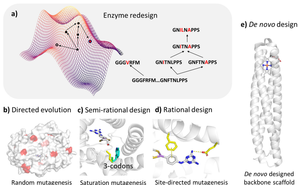
Fig. 2 Enzyme design approaches. (a) The fitness landscape map of an enzyme shows the relationship between different variants of an enzyme and their fitness (such as catalytic efficiency, thermal stability, substrate specificity, etc.). Each variant corresponds to a point on the map and the height of the point represents the fitness of the variant. (b) Directed evolution mimics the natural evolution process to improve the function of proteins through multiple rounds of random mutation, screening and selection. (c) In the semi-rational design approach, the key sites identified based on enzyme structures are mutated with saturation mutagenesis to improve the enzyme function. (d) In the rational design approach, the sites identified based on the dynamic structures and catalytic mechanism of enzyme are mutated to improve protein function. (e) De novo design methods are used to construct protein backbones from scratch to generate protein structures with new functions.
